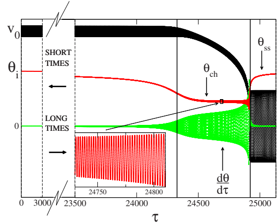
FIG. 2. (Color online) Evolution with respect to the dimensionless time \tau of the center of mass velocity v(\tau) , the orientation angle \theta(\tau) , and the angular velocity d\theta(\tau)/d\tau for \gamma=4 and the initial condition that the dimer is thrown with dimensionless initial velocity v_0=8\pi and \theta_i=1.54 . Three time regimes are seen. In the first, the center of mass velocity oscillates rapidly around a value higher than the initial value, the orientation remains close to its initial value, and the angular velocity is essentially zero. In the graph, this first regime is so long that we have shown it split into a short time part and a long time part. In the second regime, the center of mass velocity decreases in power law fashion, the orientation switches to a different constant around which it oscillates with small amplitude, and the angular velocity increases its oscillations significantly. The inset shows that the angle oscillates even where it appears to be a constant. In the third regime, the center of mass velocity changes its evolution from the power law to oscillations but now around the value zero, the amplitude of the oscillations decreasing apparently not at all or very slowly (not appreciable in the graph). In this third regime, the orientation switches to another constant value and the angular velocity vanishes. The transition between the second and third regimes is quite abrupt.
