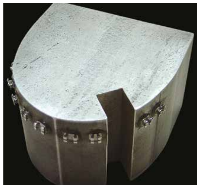
Figure 1 - Stainless steel model used in the test
