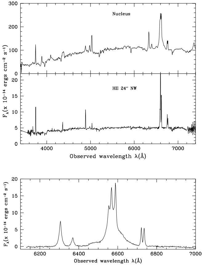
FIG. 11.— Top to bottom : Spectra of the nucleus and of an H II region 24'' northwest of the nucleus of NGC 7213, and a medium-resolution spectrum of the nucleus, after subtraction of the stellar population.
