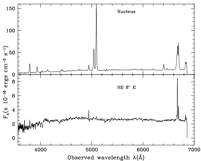
FIG. 6.—Spectra of the nucleus ( top ) and of an H II region at 8" east from the nucleus ( bottom ) of IC 1816.
