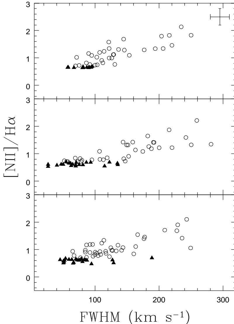
FIG. 21.—Emission-line ratio [N \text{ II}]/H\alpha plotted as a function of the FWHM of [N \text{ II}] \lambda 6584 , corrected for the instrumental FWHM. Top , NGC 1326; middle , NGC 3081; bottom , NGC 7213. Circles represent the diffuse emission, and triangles represent the H II regions. The error bars correspond to the outermost locations and represent the maximum errors in the above quantities.
