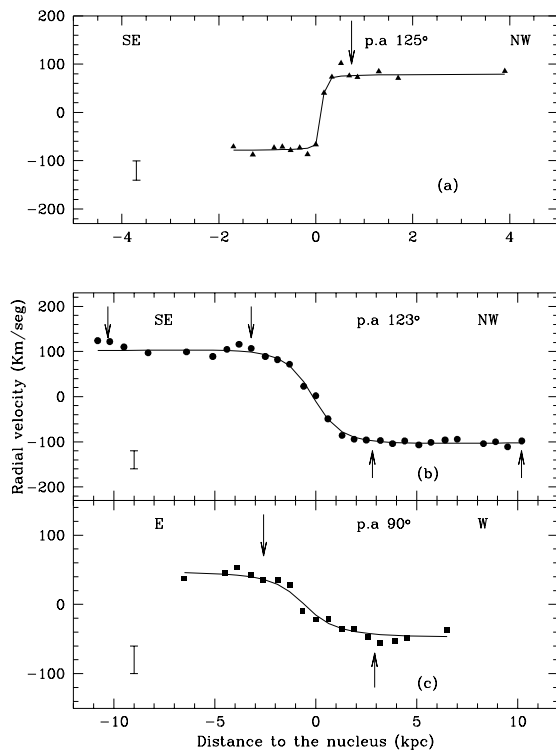
FIG. 16.—Rotation curves for NGC 1386 (top), NGC 1598 (middle), and IC 1816 (bottom). The locations of the H II regions (in spiral arms in at least NGC 1386 and NGC 1598) are indicated by arrows. The error bars represent the maximum uncertainty in the individual velocity measurements ( \approx 15 \text{ km s}^{-1} ).
