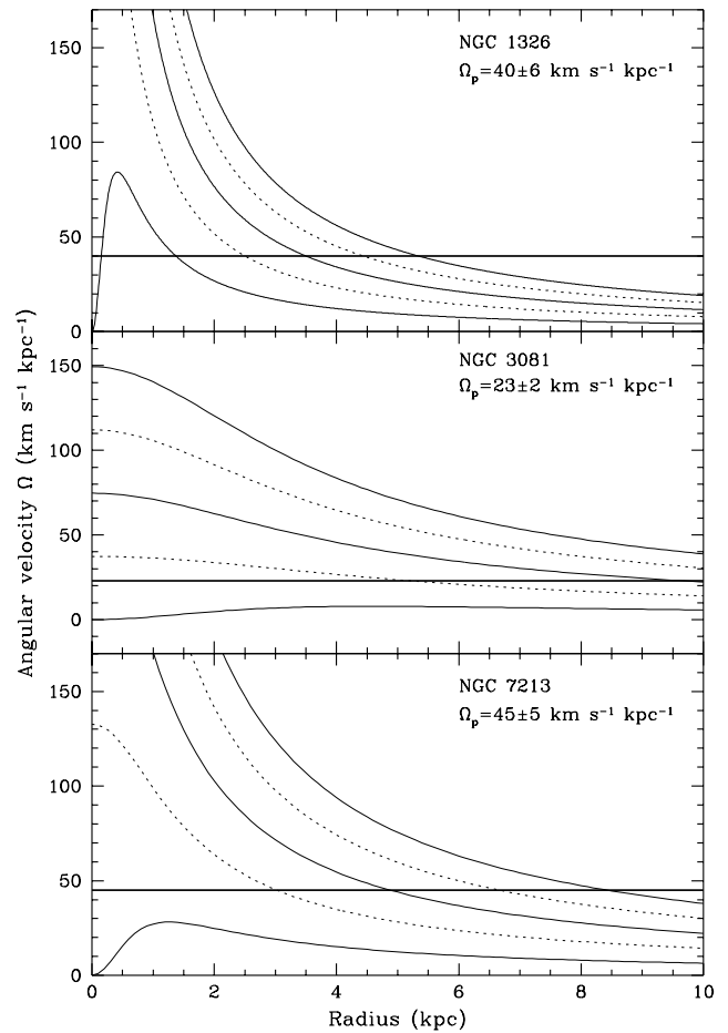
FIG. 17.—Angular velocities \Omega and Lindblad curves \Omega \pm \kappa/2 (solid lines) and \Omega \pm \kappa/4 (dotted lines) obtained from the kinematic models fitted to the data. \Omega_p (heavy solid lines) is the pattern speed of the bar in NGC 1326 and NGC 3081 and of the spiral arms in NGC 7213 (see § 5).
