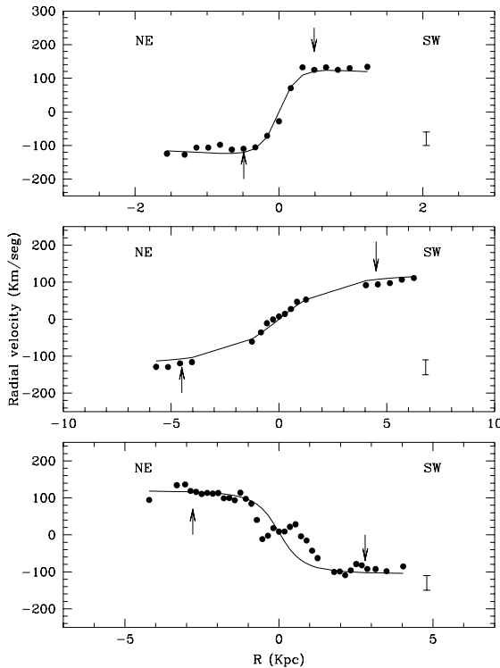
FIG. 15.—Rotation curves along the slit position through the nucleus for NGC 1326 (top), NGC 3081 (middle), and NGC 7213 (bottom), together with the best circular model. The locations of the star-forming rings are indicated by arrows. The error bars represent the maximum uncertainty in the individual velocity measurements ( \approx 15 \text{ km s}^{-1} ).
