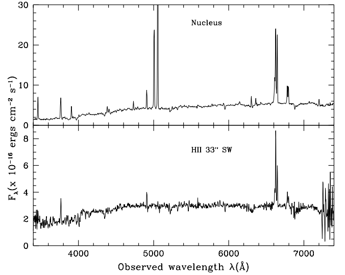
FIG. 10.—Spectra of the nucleus ( top ) and of an H II region at 33" southwest from the nucleus of NGC 3081.
