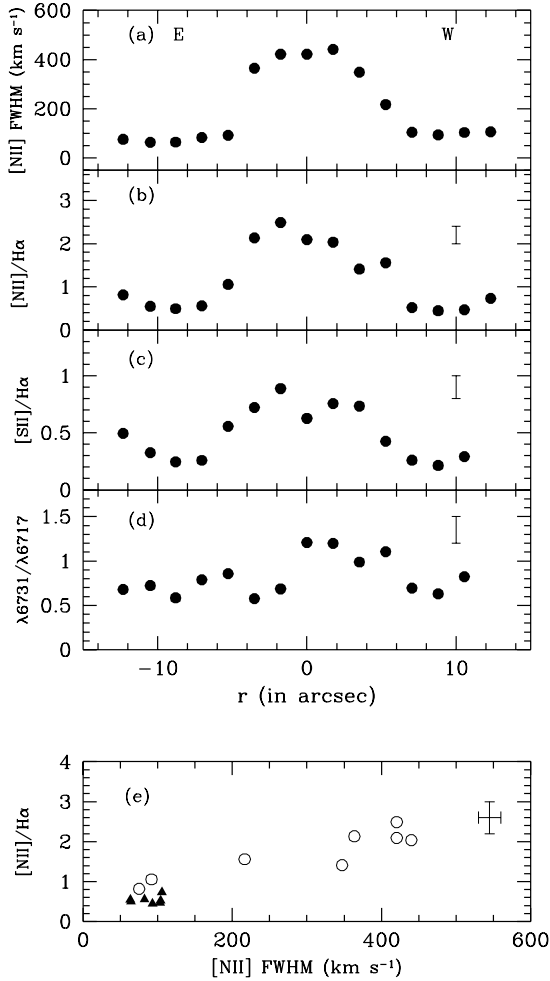
FIG. 22.—Top to bottom: FWHM of [N II] \lambda 6584 , corrected for the instrumental FWHM, and the emission-line ratios [N II]/H \alpha , [S II]/H \alpha , and [S II] \lambda 6731/\lambda 6717 plotted as a function of distance from the nucleus for IC 1816. The lower panel shows [N II]/H \alpha plotted against [N II] FWHM; open circles represent the diffuse emission, and triangles represent the H II regions. The error bars correspond to the outermost locations and represent the maximum errors in the above quantities.
