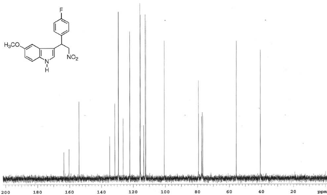
Figure S32. ^{13}\text{C} NMR ( \text{CDCl}_3 ) of compound 5j .
