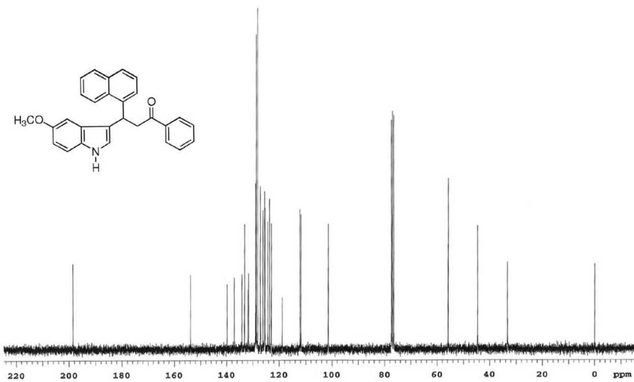
Figure S20. 13 C NMR (CDCl 3 ) of compound 3w.
