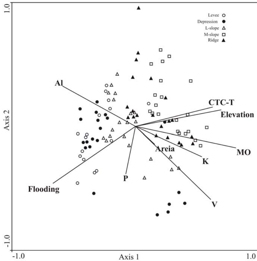
Figure 4. Ordination biplot depicting the two axes of the environmental partial CCA of sampling units in a riverine forest in Southern Brazil. Each sampling unit was identified by different symbols according to the respective transect. Environmental variables are represented their acronyms (see Table 2).
