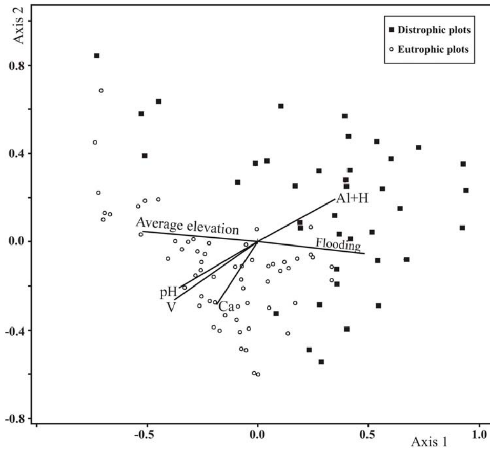
Figure 4. Ordination biplots diagram of plots and environmental variables (vectors) of the first two ordination axes yielded by canonical correspondence analysis (CCA) based on those species > 10 individuals surveyed on the riverside forest of Rio Botucaraí, Cachoeira do Sul, Southern Brazil.
