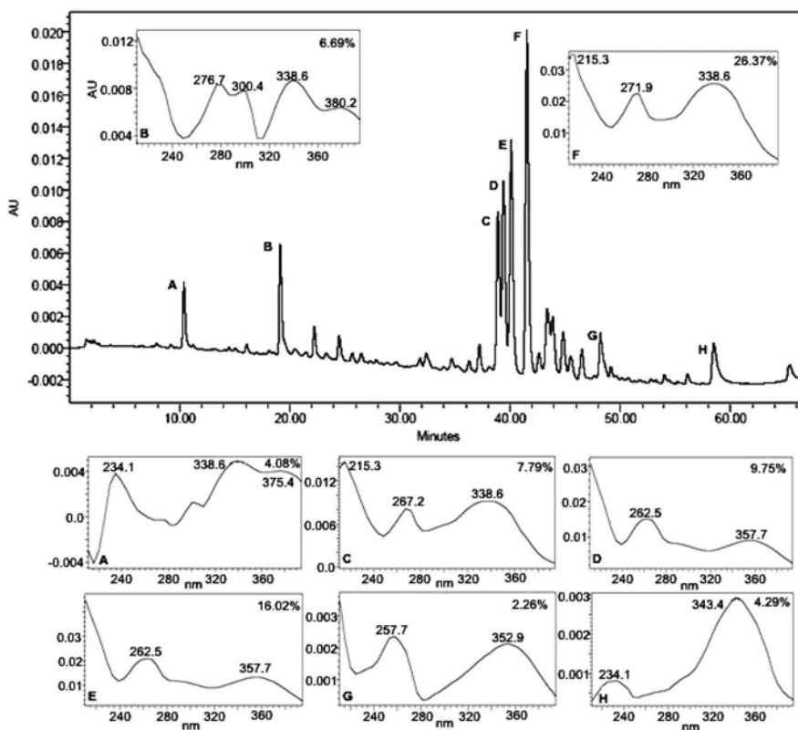
Fig. 5. HPLC Profile of AEBM Detected at 356 nm
