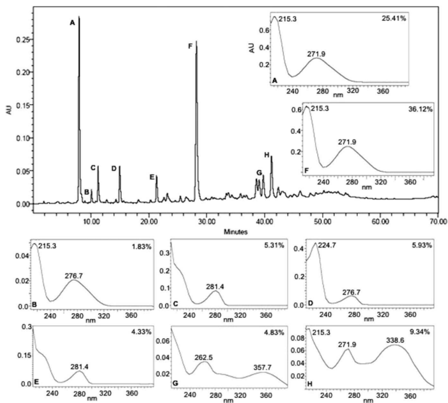
Fig. 4. HPLC Profile of HEBM Detected at 270 nm
