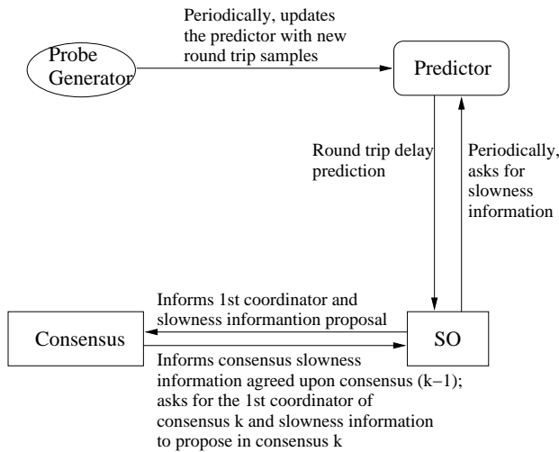
Figure 1: An adaptive consensus protocol supported by a predictor-based slowness oracle
