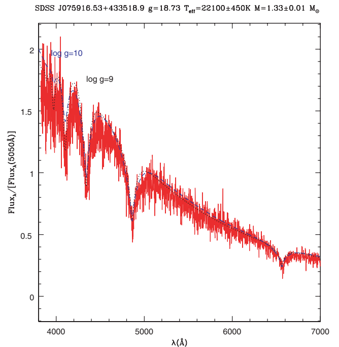
Figure 10. Spectrum of SDSS J075916.53+433518.9 with g = 18.73 , T_{\text{eff}} = 22\,100 K and two models, with \log g = 9 and 10. The higher \log g fits the H\alpha line better, but the lower \log g fits the higher lines better, where the SNR is smaller. This low SNR is typical for the stars closer to our upper cut-off of g = 19 .
