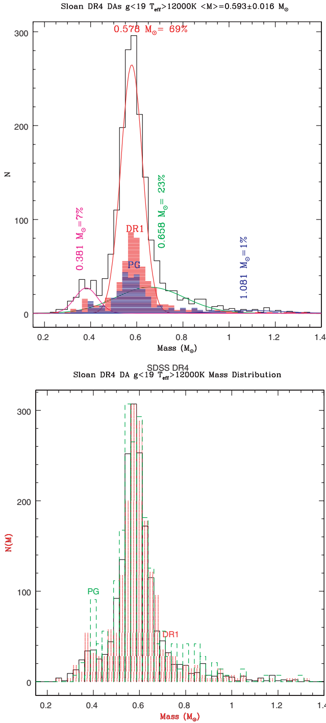
Figure 1. Histogram for the 1859 DA stars brighter than g = 19 and hotter than T_{\text{eff}} = 12000 K, compared to the PG survey published by Liebert et al. (2005) and the SDSS DR1 sample published by Madej et al. (2004). Gaussian fits detailed in Table 1 are also shown. Our bins are 0.025 M_{\odot} wide. The second graph shows the DR1 and PG survey data normalized to the DR4 sample, even though those samples are smaller and therefore have significantly larger error bars.
