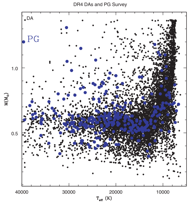
Figure 2. Masses for all 3595 DA white dwarf stars brighter than g = 19 and cooler than 40000 K, showing an increase in mean mass for lower T_{\text{eff}} . The large solid (blue) circles are the values published by Liebert et al. (2005), showing the increase in mass at lower T_{\text{eff}} is also present in their sample, which uses a totally independent grid of models and fitting technique.
