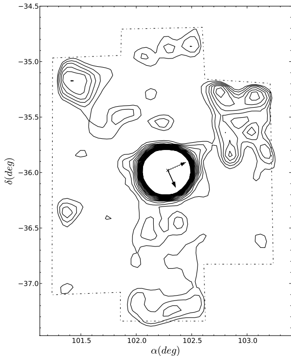
Figure 8. The result of applying the MF to NGC 2298 CTIO data. We show the derived number of stars, \gamma_{cl} , in a contour plot. The first three contour levels correspond to 0.8, 1.8, 2.8 \sigma above background. The inner contours start at the tidal radius of the cluster. The dashed arrow points to the direction perpendicular to the Galaxy disc. The solid line points towards the proper motion direction (Dinescu et al. 1999). The resulting map was smoothed using a 0 ^{\circ} 06 Gaussian kernel, thus enhancing structures with a typical size similar to r_t .
