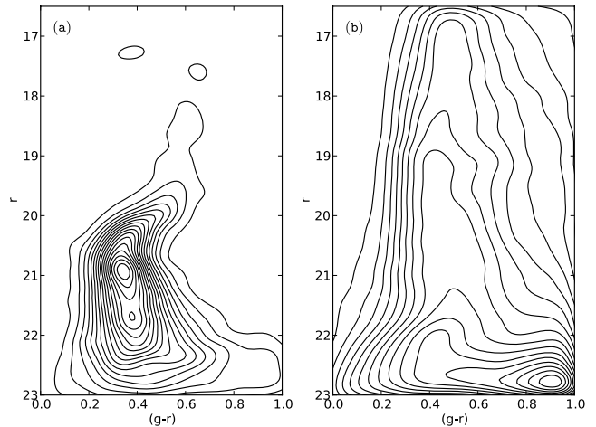
Figure 3. Panel (a): r , (g - r) F_{cl} contours on the CMD plane for the Palomar 5 SDSS data. Panel (b): same as in panel (a) but now showing the F_{bg} contours. In both panels the contour levels are normalized to the range varying from 0 to 1, and are evenly spaced by 1/20 .
