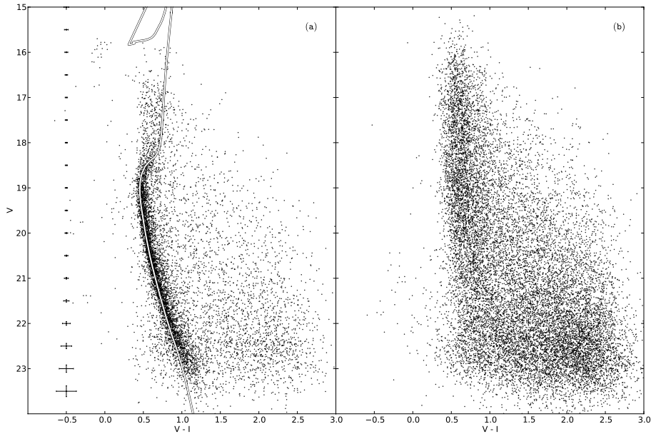
Figure 6. Panel (a): V , (V - I) CMD of NGC 2298 where only stars inside r = 37 pc were chosen. The mean photometric error is shown in the extreme left of this panel. We also show the best-fitting isochrone with (m - M) = 15.15 and the (V - I) offset of 0.06 explained in the text. Panel (b): V , (V - I) CMD for stars outside r = 37 pc. Only 10 per cent of the total stars are shown for clarity.
