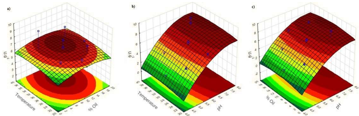
Figure 1. Response surfaces from CCD analysis of 96 h cultivation, of Aspergillus brasiliensis in malt bagasse, where (a) is influence of temperature and % of oil, (b) is influence of temperature and pH, and (c) is influence of % of oil and pH in lipase activity. Experiments were run using the static flat-bed bioreactor configuration.
