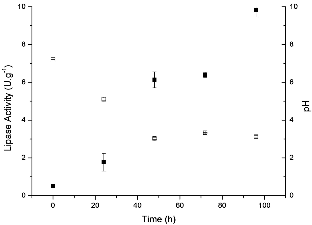
Figure 5. Lipase activity (■) and pH (□) profiles of SSC of Aspergillus brasiliensis 157f in plugged-flow bed with forced water-saturated aeration bioreactors (malt bagasse).
