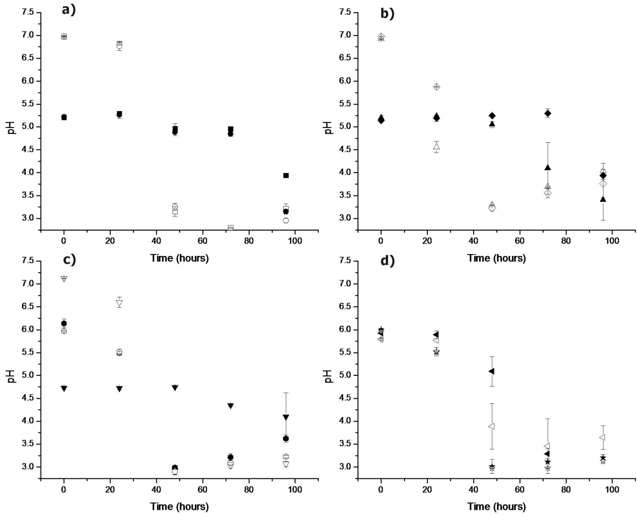
Figure 3. Kinetics of pH variation during the CCD experiment for Aspergillus brasiliensis 157f cultivation in the static flat-bed bioreactor configuration. Panels (a): treatments A (■), B (□), C (●), and D (○); (b): treatments E (▲), F (△), G (◆), and H (◇); (c): treatments I (▼), J (▽), K (●), and L (○); and (d): treatments M (◄), N (◁), O (★), and P (☆).
